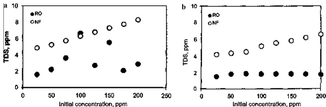
Figure 7 Concentration of (a) Cu(II) and (b) Cd(II) ions in the permeate from RO and NF (Abu Qdaia and Moussab, 2004).
